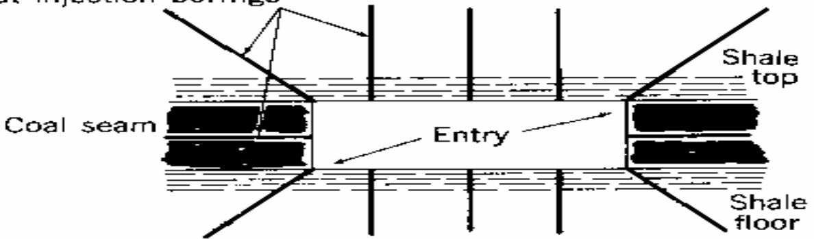
Fig. 2B - Section through entry
